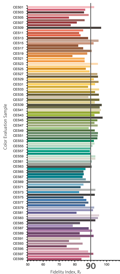
Okalite Standard LED 3000K R_f = 84
