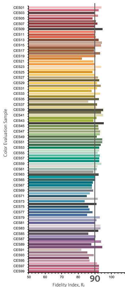
Okalite EFFICIENT WHITE R_f = 91
